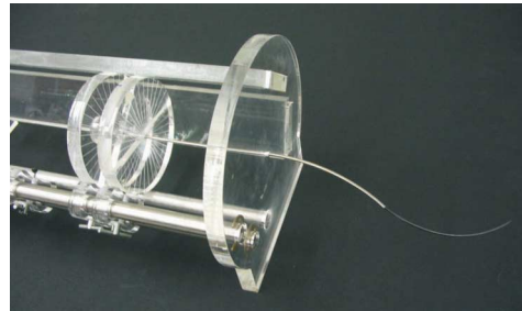
Fig. 9. Manual actuation mechanism. Both tube and wire have input circular handles etched to encode rotation and the support structure features a linear ruler etched to encode translation. Spring pin locking mechanisms hold the wheels at desired linear and angular positions.
