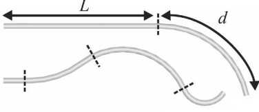
Fig. 5. (Top) Tubes used in all active cannula studies to date (including this paper) consist of a straight transmission of length L , with a constant curvature section of length d at one end. (Bottom) Our models presented here are, in principle, general enough to account for piecewise circular/straight tubes with multiple transition points.
